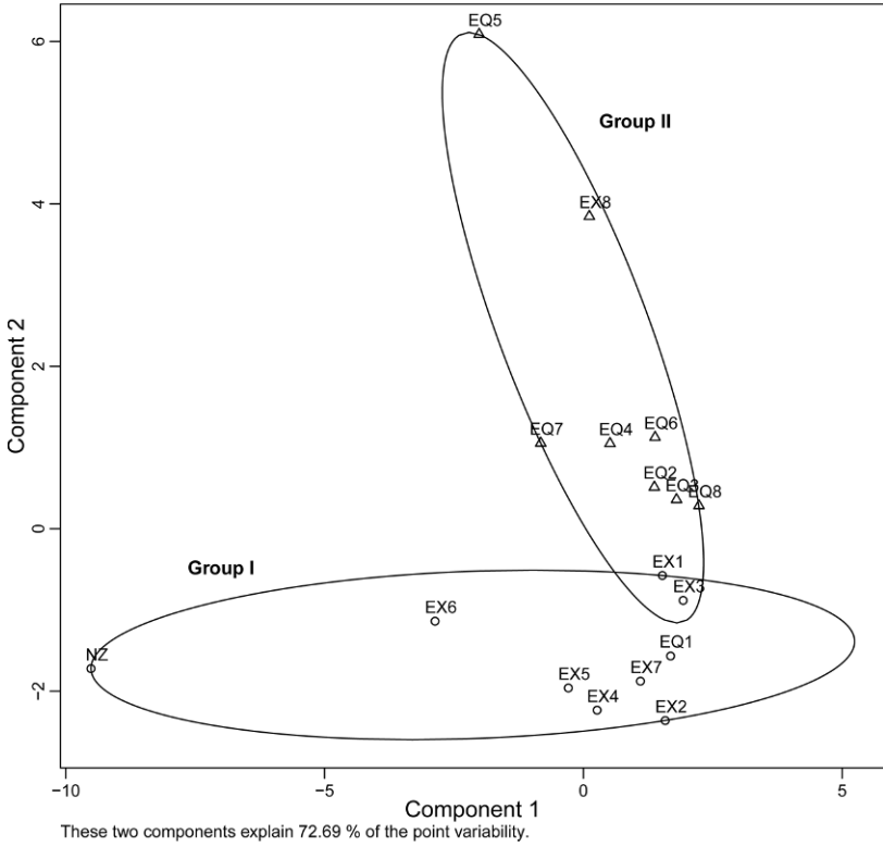
Fig. 7.16. Clustering results for the earthquake and explosion series based on symmetric divergence using a robust version of k-means clustering with two groups. Circles indicate Group I classification, triangles indicate Group II classification.
