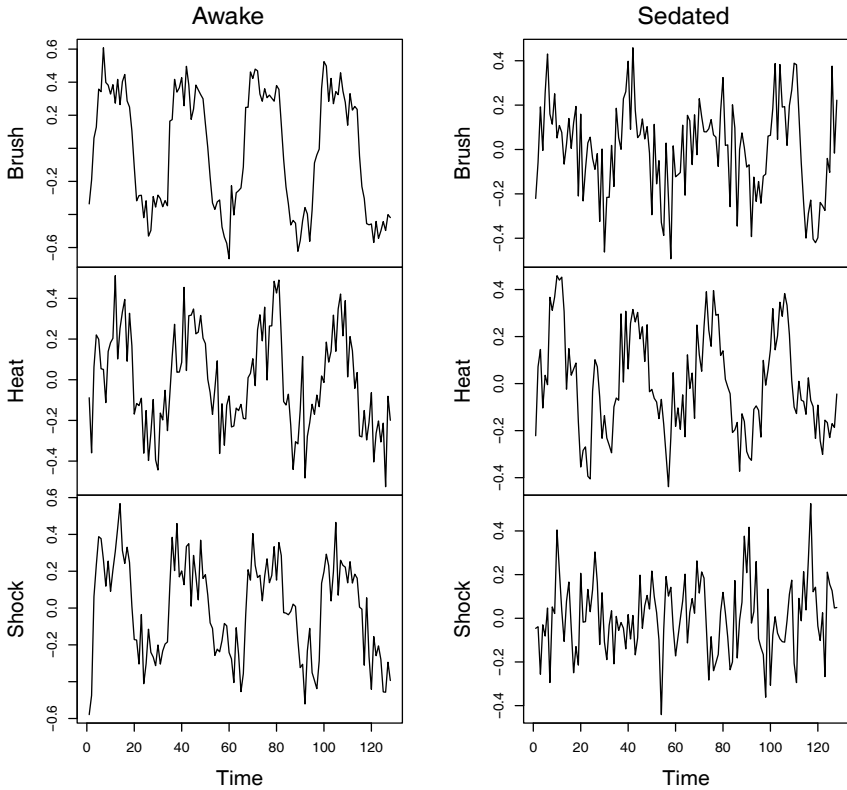
Fig. 7.1. Mean response of subjects to various combinations of periodic stimulae measured at the cortex (primary somatosensory, contralateral). In the first column, the subjects are awake, in the second column the subjects are under mild anesthesia. In the first row, the stimulus is a brush on the hand, the second row involves the application of heat, and the third row involves a low level shock.
