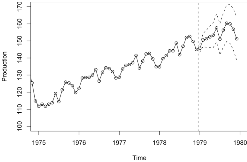
Fig. 3.26. Forecasts and limits for production index. The vertical dotted line separates the data from the predictions.
