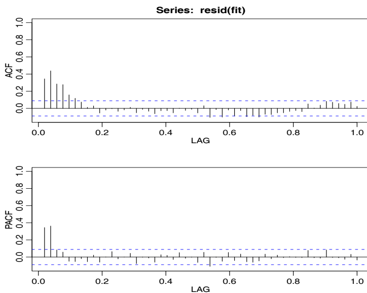
Fig. 5.9. Sample ACF and PACF of the mortality residuals indicating an AR(2) process.
