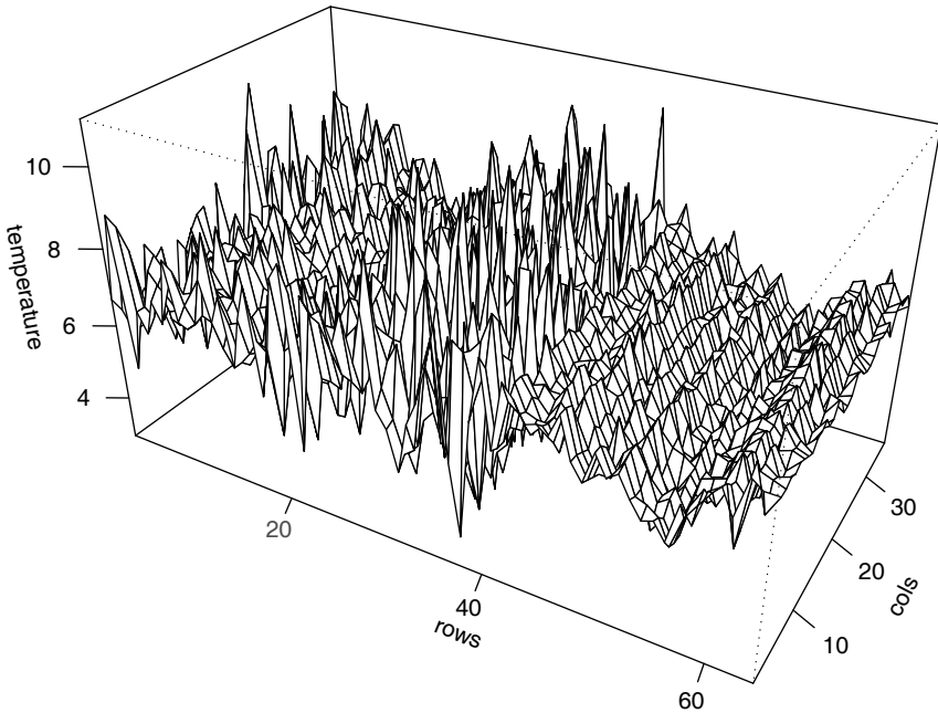
Fig. 1.15. Two-dimensional time series of temperature measurements taken on a rectangular field ( 64 \times 36 with 17-foot spacing). Data are from Bazza et al. (1988).
