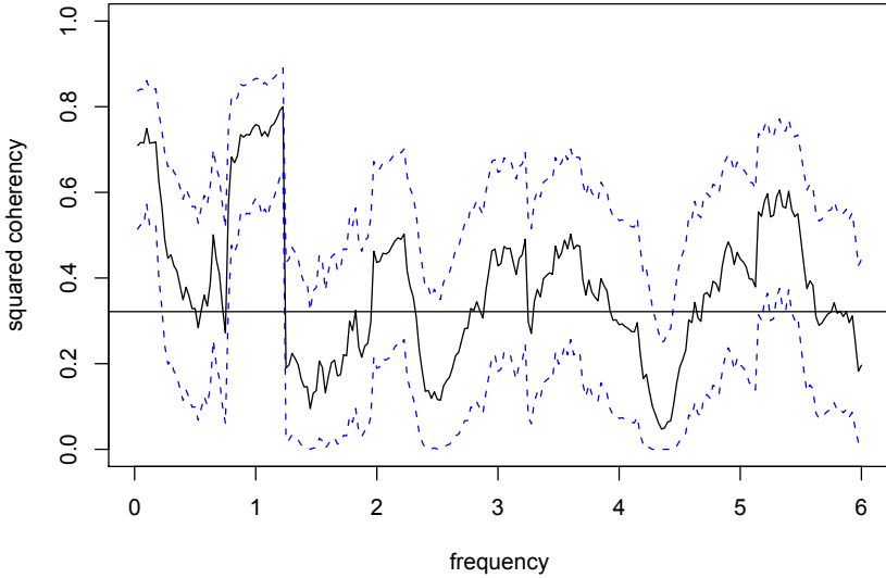
Fig. 4.13. Squared coherency between the SOI and Recruitment series; L = 19 , n = 453 , n' = 480 , and \alpha = .001 . The horizontal line is C_{.001} .
